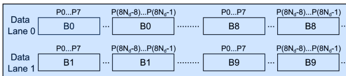
Fig. 15: The defense of grouped pixel smoothing where the same bits from 8N_d adjacent (similar) pixels are transmitted together to minimize bit flip-caused EM emissions.
