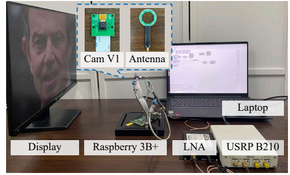
Fig. 16: The experiment setup for the feasibility tests.
