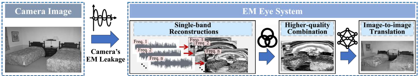
Fig. 7: The image eavesdropping pipeline of EM Eye.
